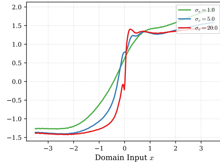
(f) Neural Network: Variasi Bobot \sigma_v
